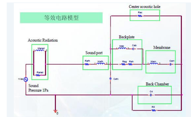
Equivalent Circuit Model
