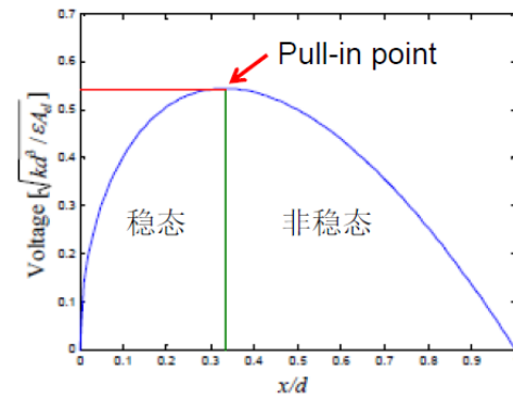
Pull-in Voltage Simulation & CV Measurement
