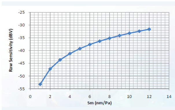
Sensitivity Sm Simulation
